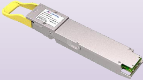
1600G OSFP2xDR4
